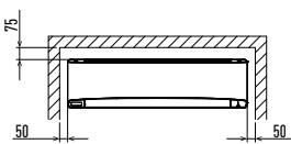
Montageabstand
