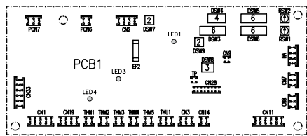
PCB1 Sockets Location
