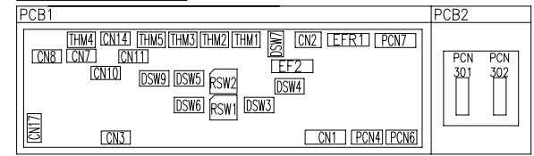
Printed Circuit Board
